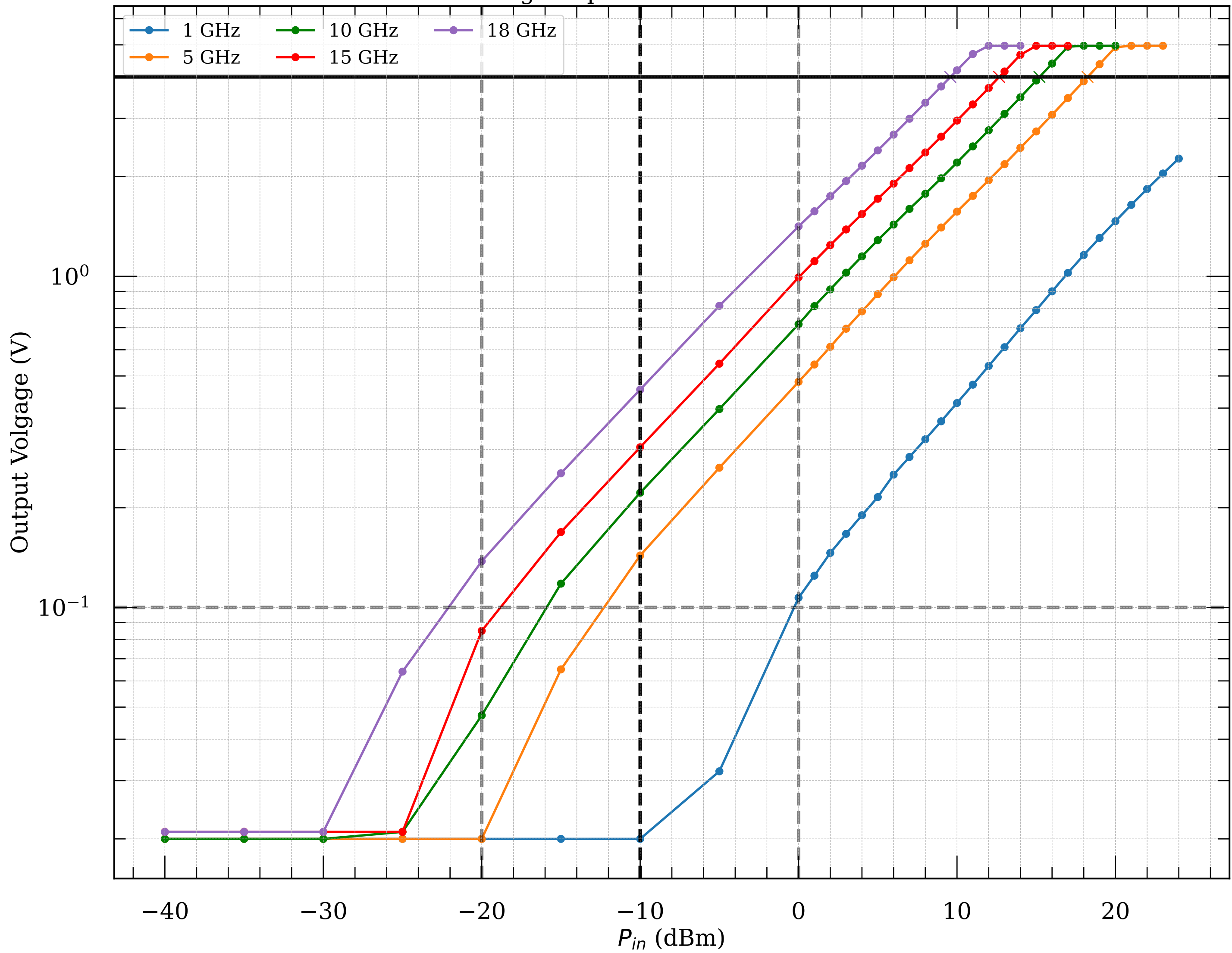
Measured voltage-to-power curve of detector module084
